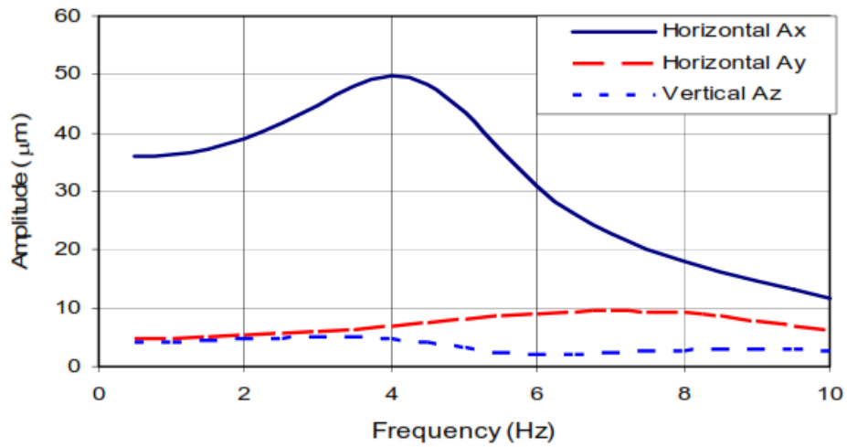
Fig.5. Rigid Structure Rest on Flexible Piles
