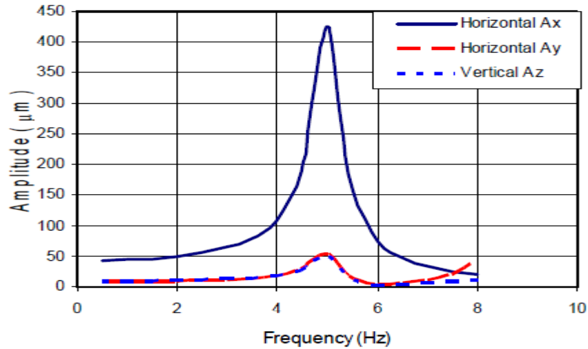
Fig. 4 Dynamic Response of Structure with Soil-Pile-Structure Interaction
